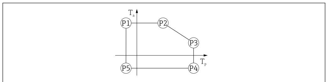
■ 26 铝外壳材质; 过程温度范围: -40 \dots +200 \text{ }^{\circ}\text{C} ( -40 \dots +392 \text{ }^{\circ}\text{F} )
